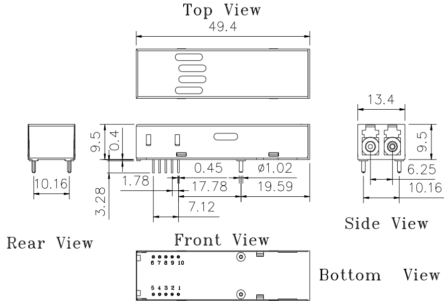
TRSL-9140G / TRSL-9140AG
