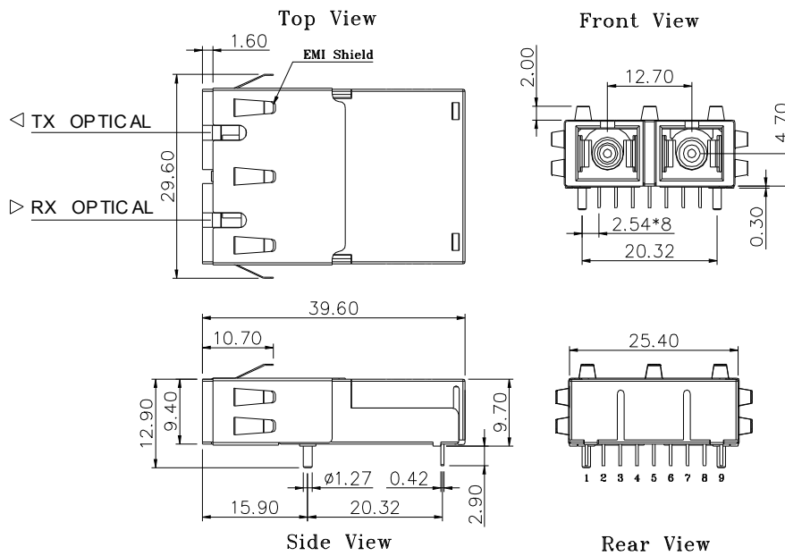
TRS-5380-CXX0-EMG / TRS-5380C-CXX0-EMG
