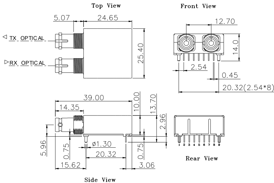
TRS-5380T-CXX0G / TRS-5380CT-CXX0G
